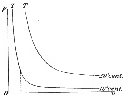
FIG. 2.—Isotherms.
